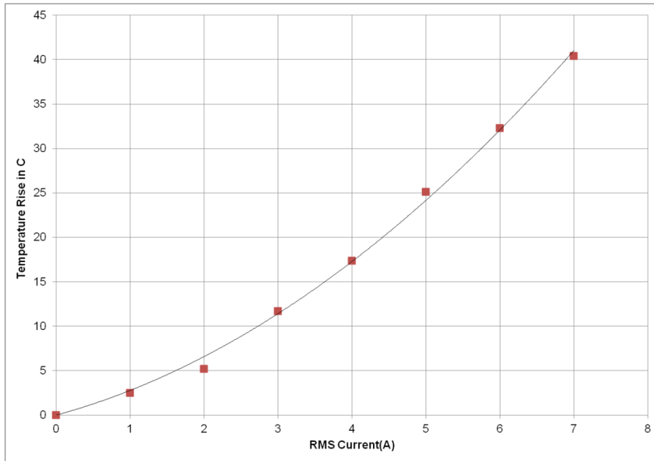
Fig 12: Temperature rise in GS206 with RMS current
