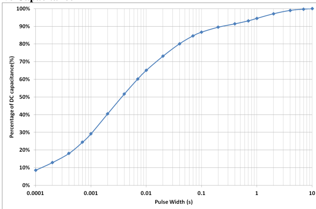
Figure 4: Effective Capacitance
